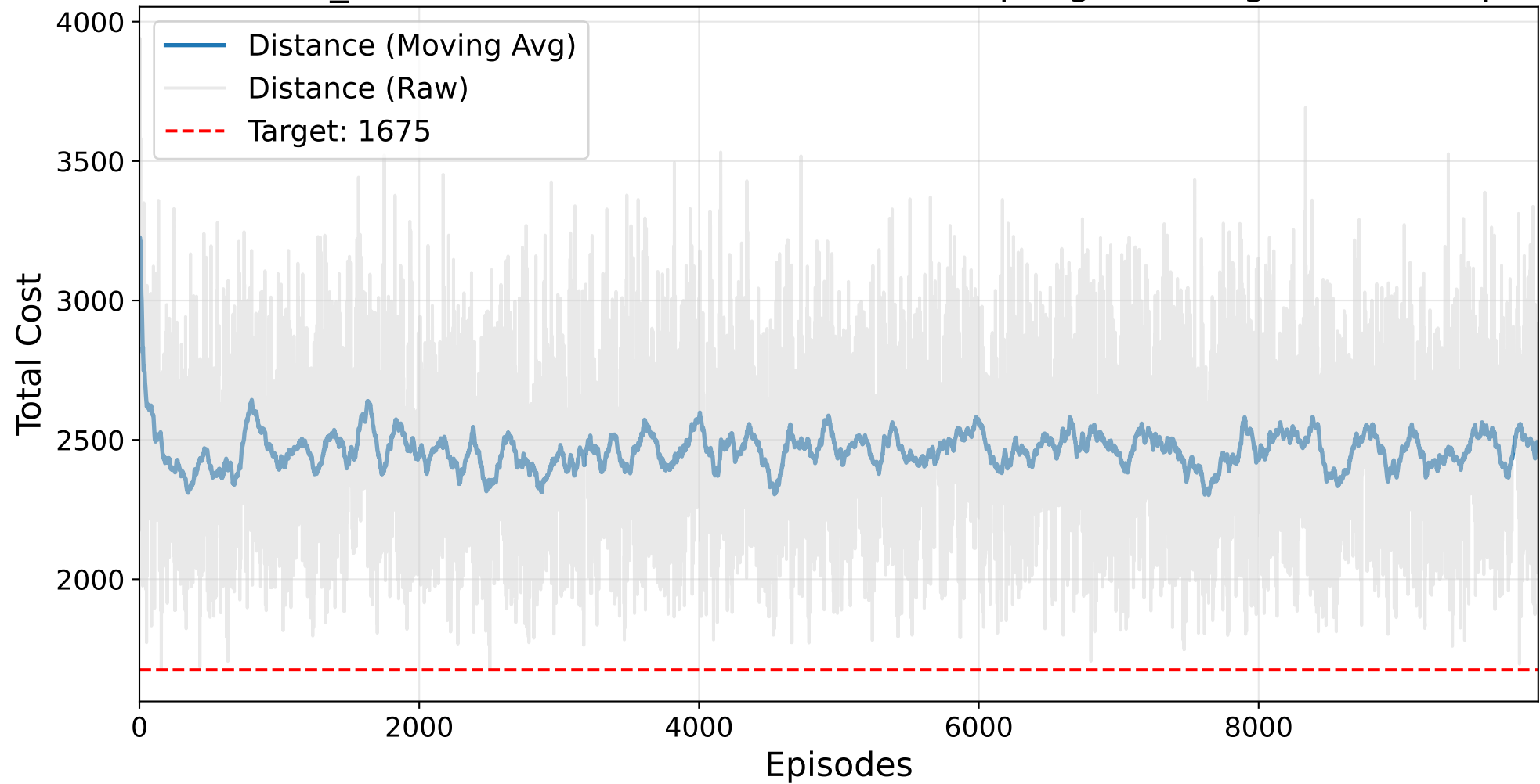
Final NO_MASK Masked AutoRL-SOP (Resampling) Training - ESC12.sop
